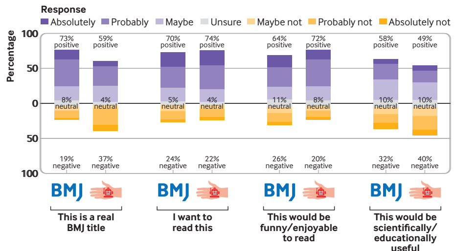
Fig 3 | Real titles of Christmas research articles in The BMJ compared with curated top 10 ranked AI generated titles using seven point Likert scales
